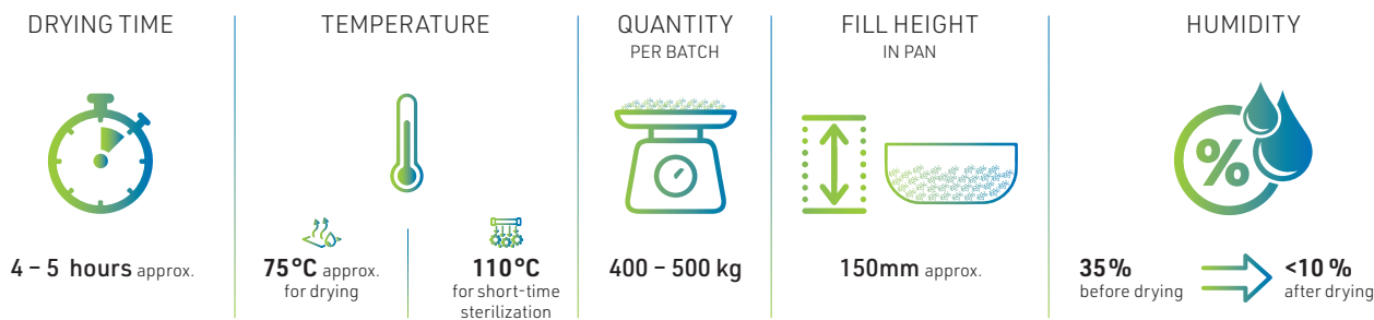
Comprehensive view of Aust & Hachmann drying parameters
